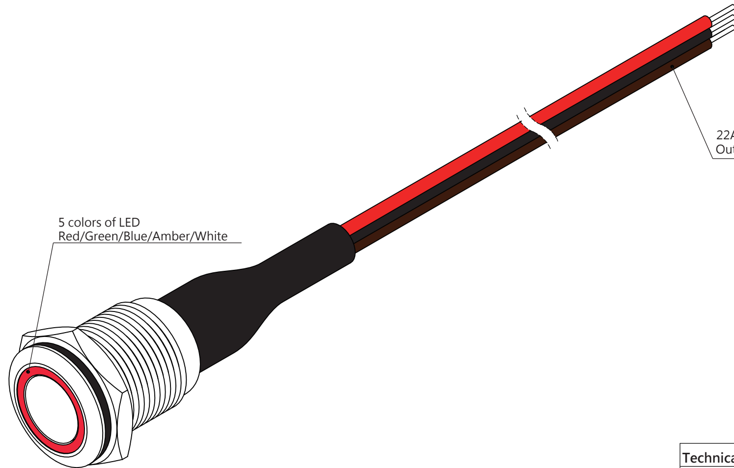
ISOMETRIC VIEW
