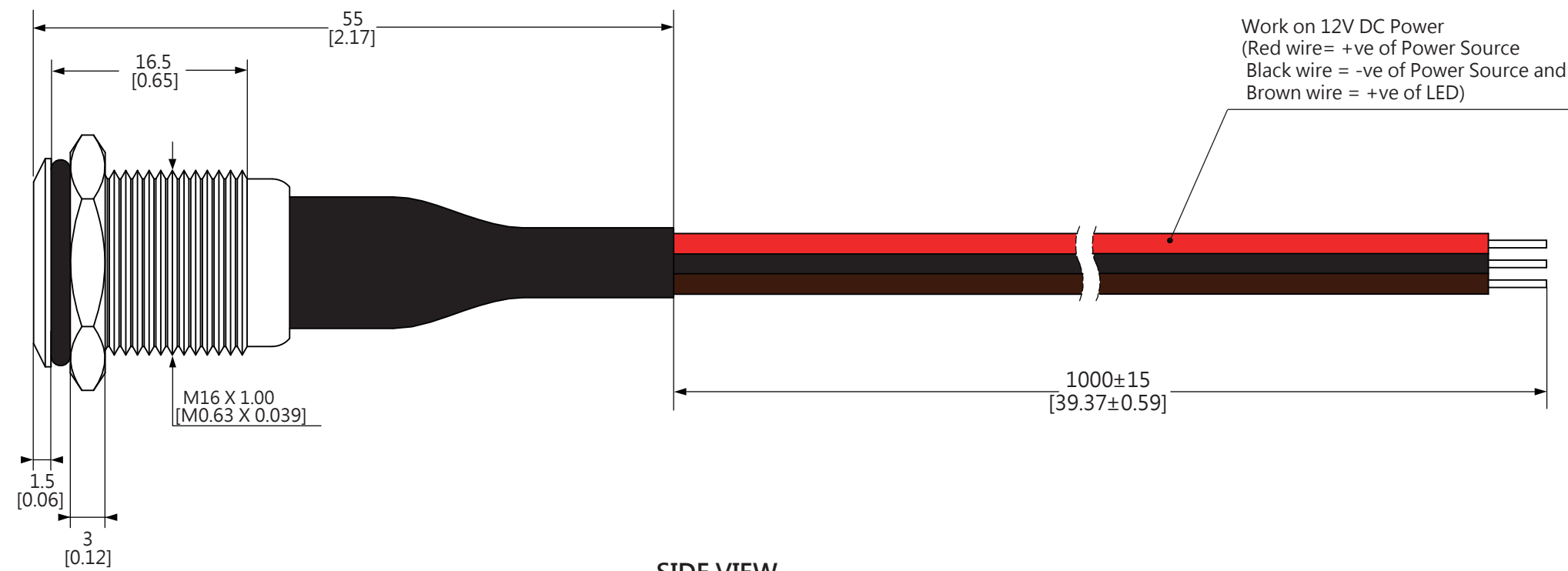
SIDE VIEW
