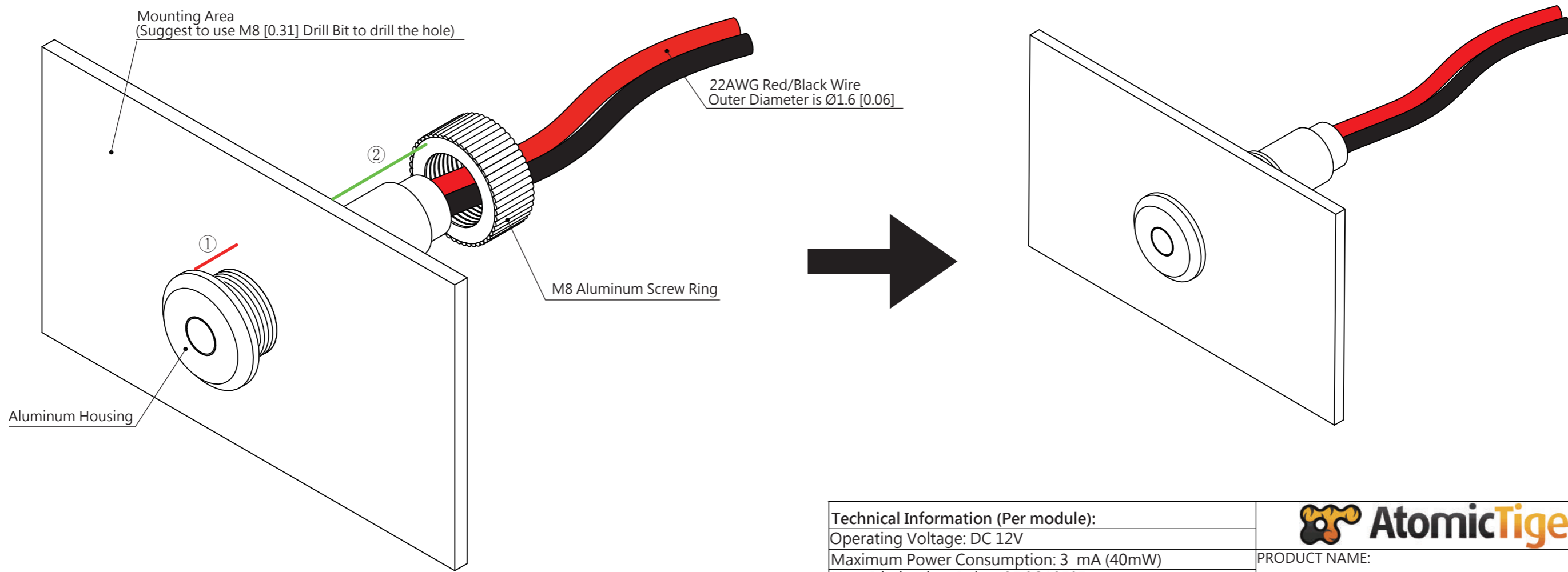
INSTALLATION DIAGRAM
