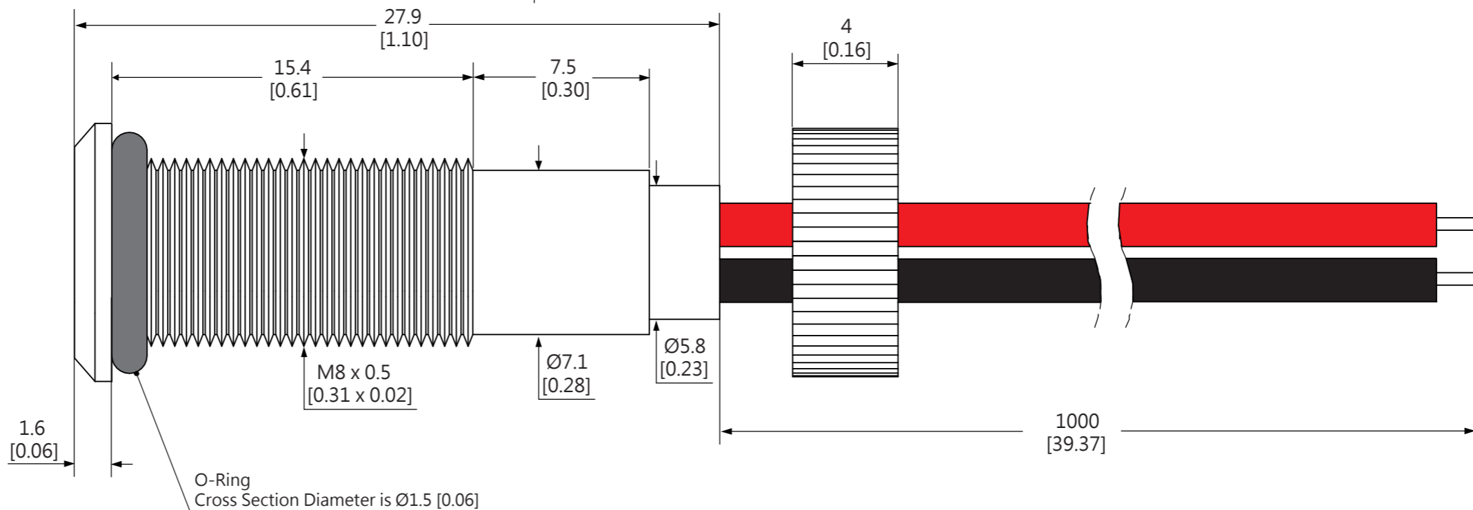
SIDE VIEW
