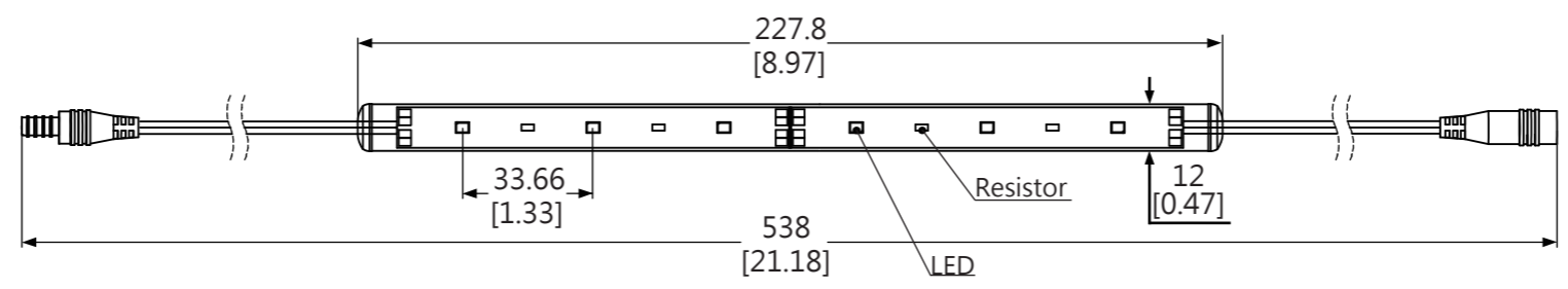
TOP VIEW
